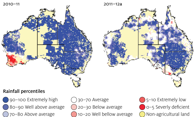
MAP 2 Australian rainfall percentiles
